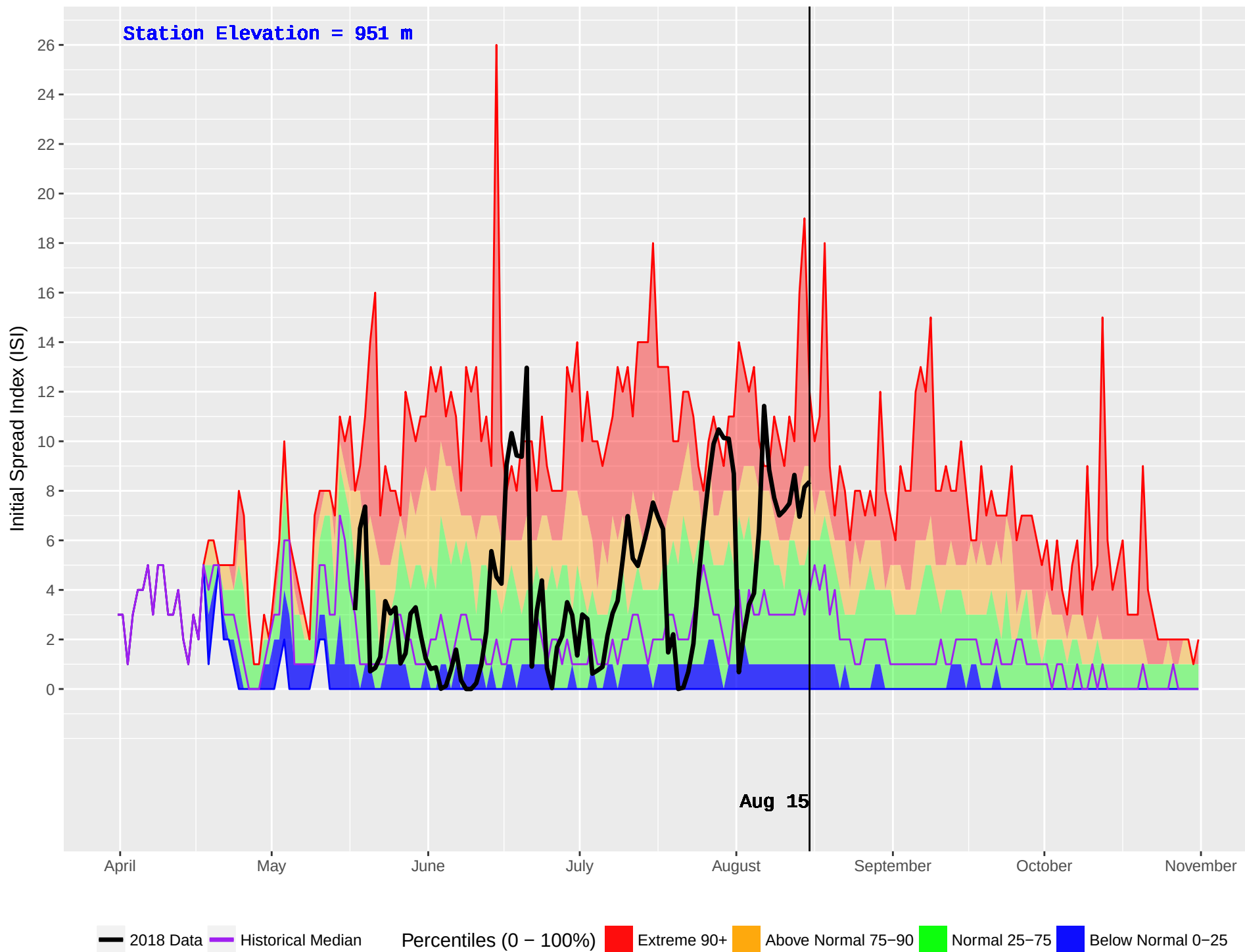
NORTH BABINE (173) : Historical (1986–2016) and Current (2018) Daily Initial Spread Index (ISI)
