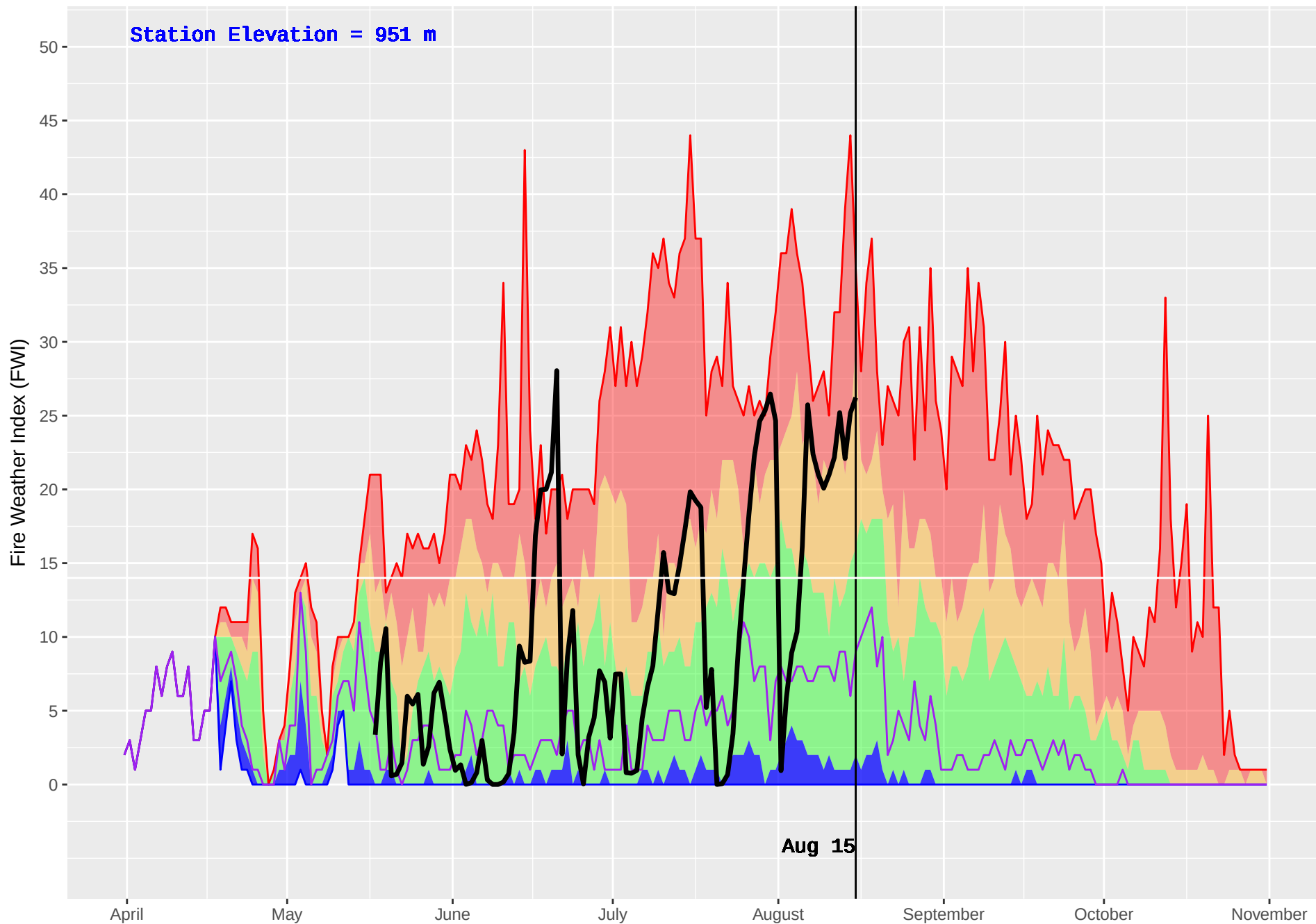
NORTH BABINE (173) : Historical (1986–2016) and Current (2018) Daily Fire Weather Index (FWI)
