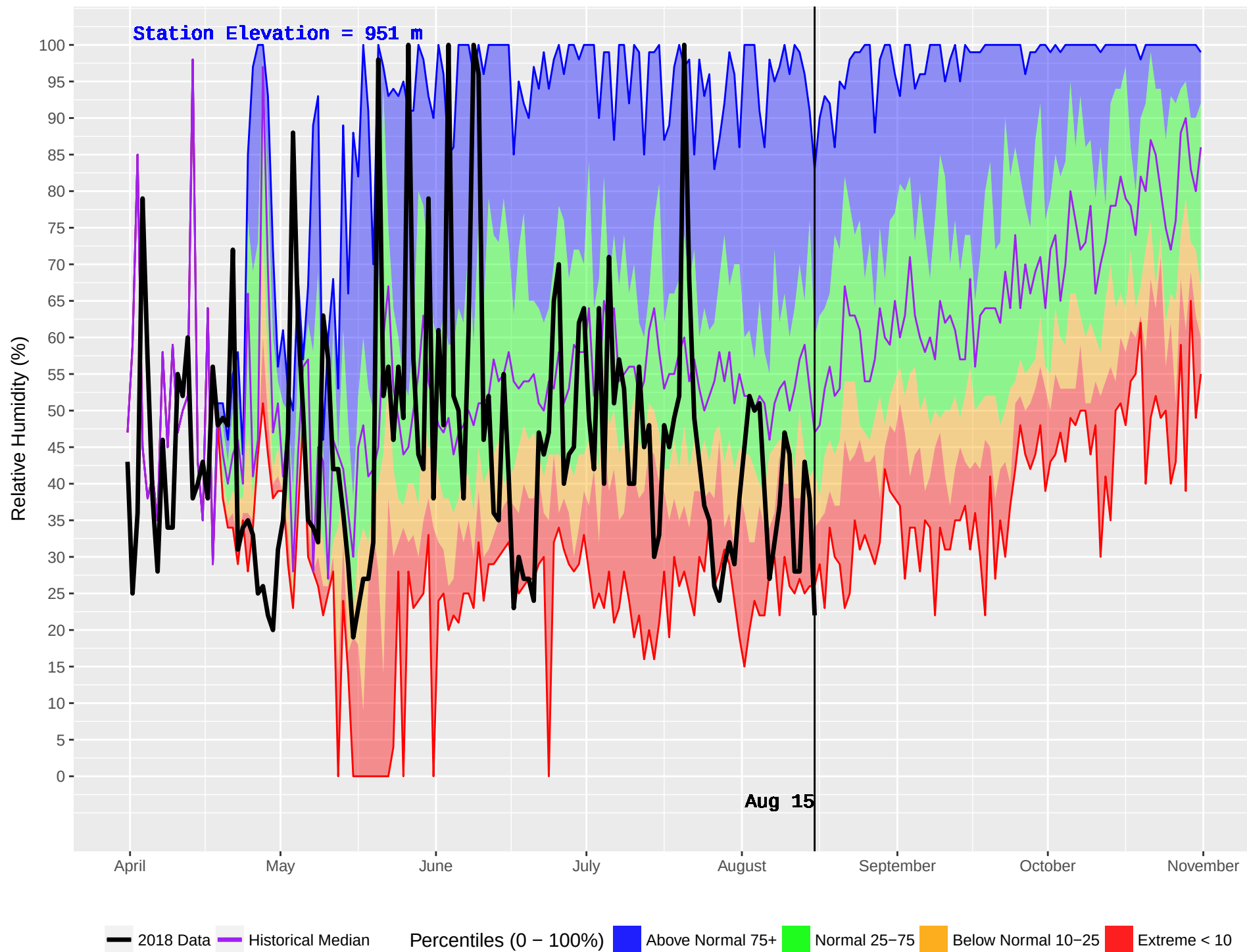
NORTH BABINE (173) : Historical (1986–2016) and Current (2018) Daily Relative Humidity
