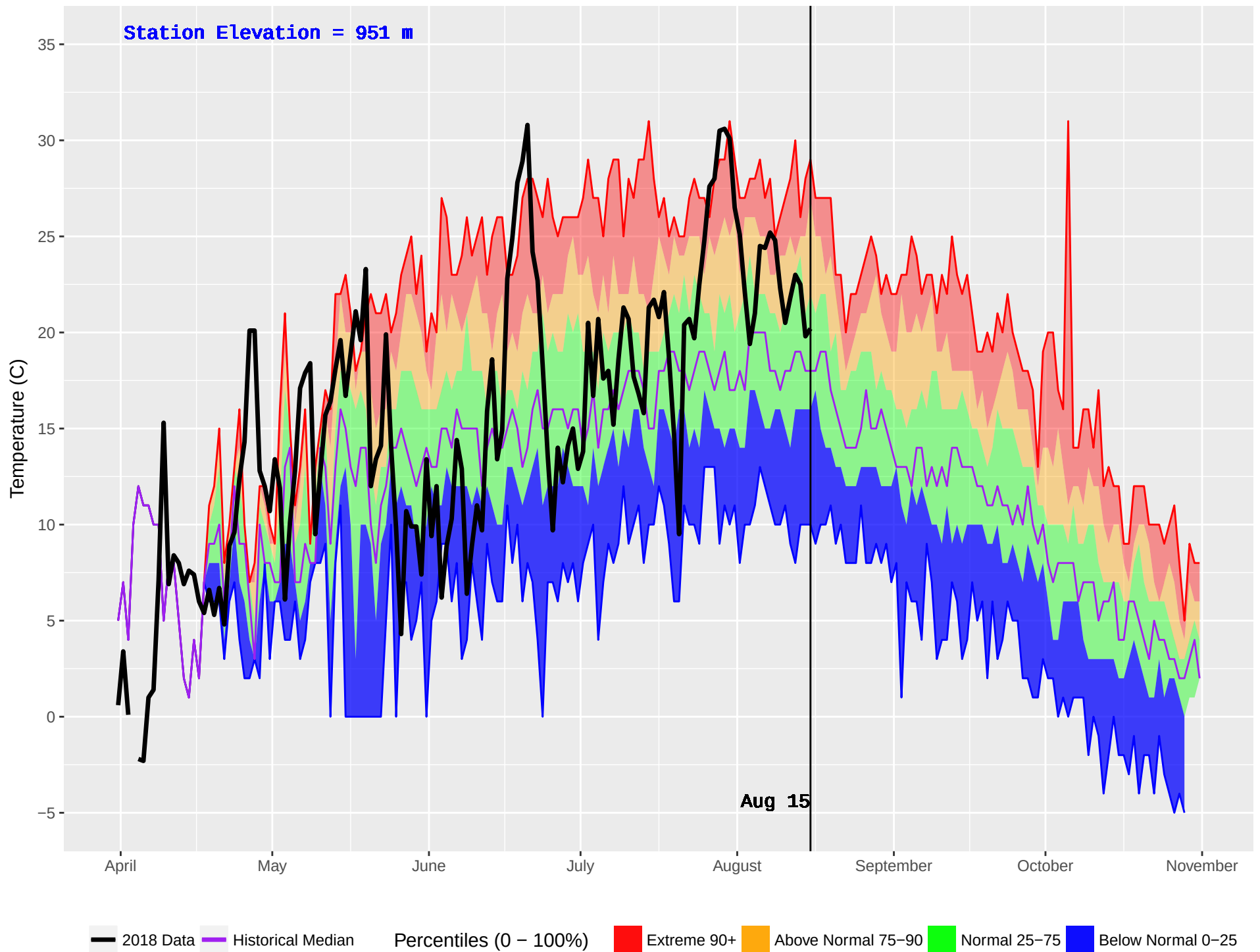
NORTH BABINE (173) : Historical (1986–2016) and Current (2018) Daily Temperature
