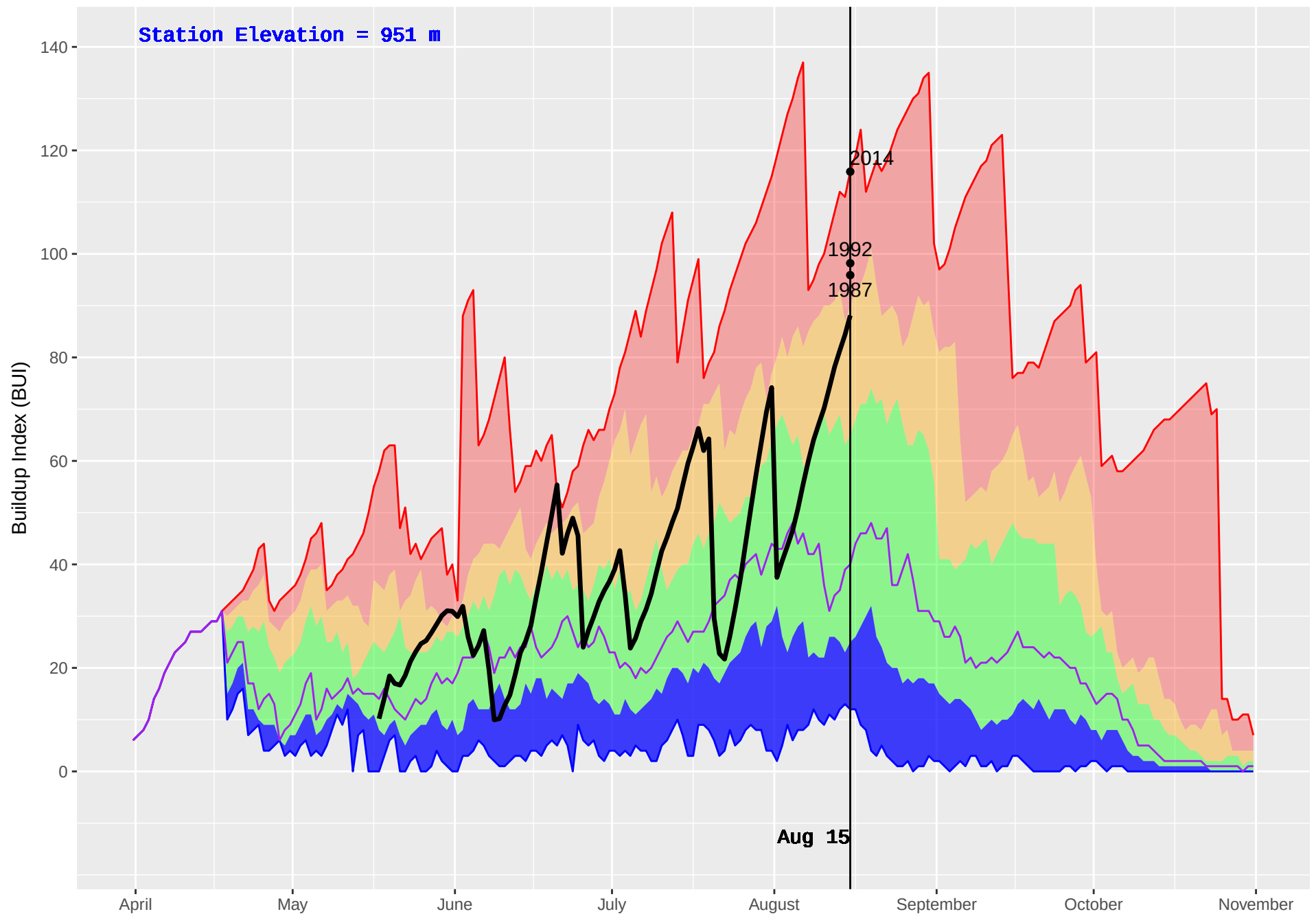
NORTH BABINE (173) : Historical (1986–2016) and Current (2018) Daily Buildup Index (BUI)
